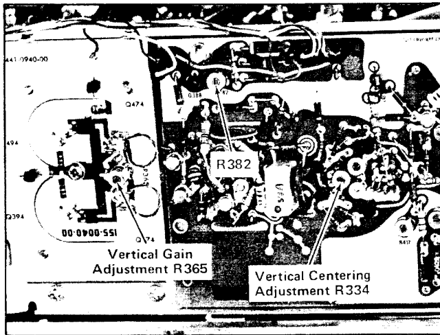
Fig. 5-8. Location of Vertical Output Amplifier Centering and Gain adjustments and R382.
