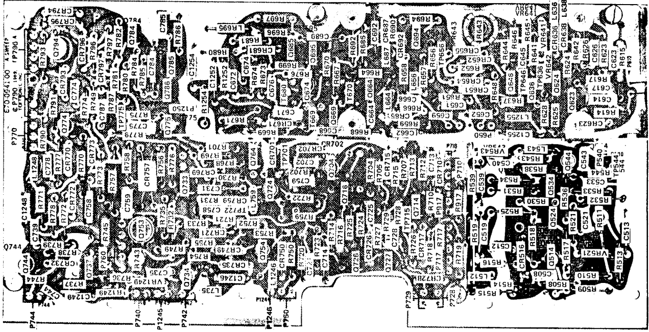
Fig. 8-6. Partial A Sweep circuit board—P/O A4. Trigger Preamp circuit shown.
